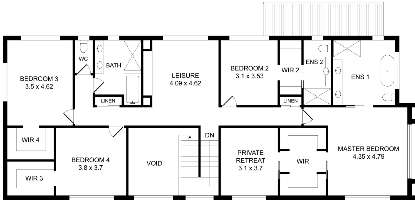
UPPER FLOOR
